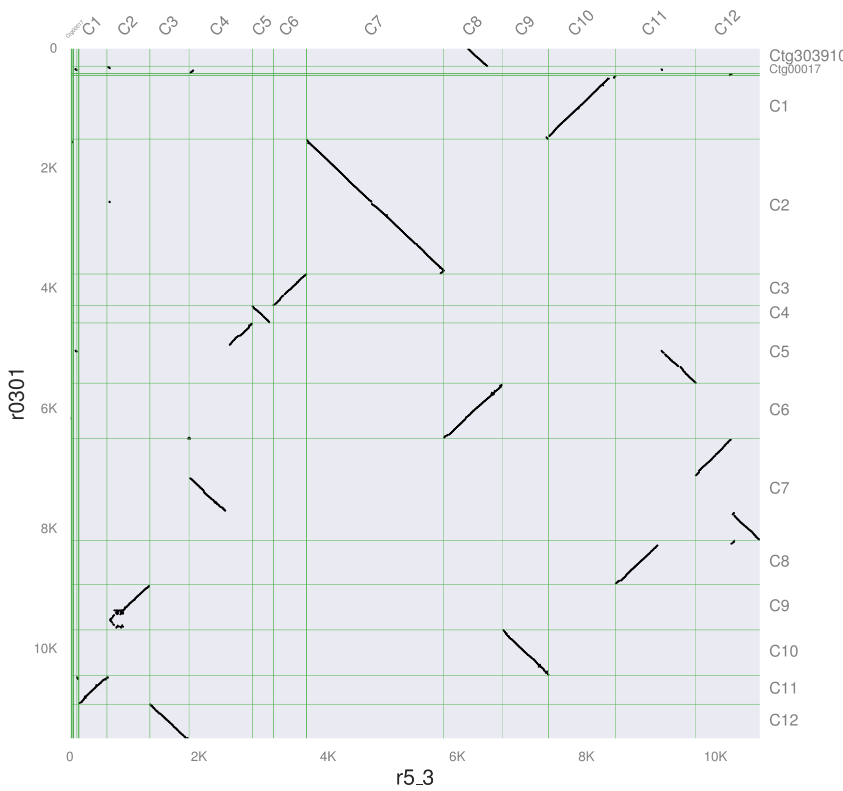
Inter-genomic comparison: r5_3 vs r0301 (5,061 gene pairs)
